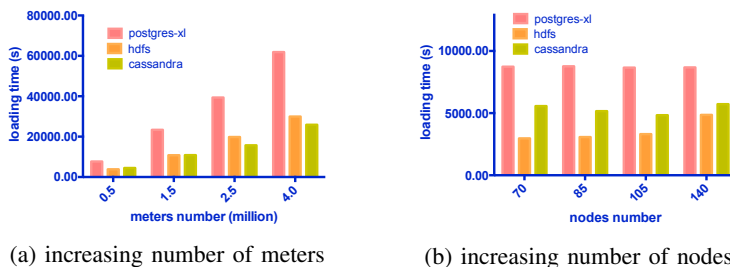
Fig. 2: Data loading
