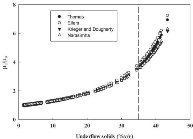
Fig. 5. Underflow enhanced viscosity comparison within 4 different viscosity model.
