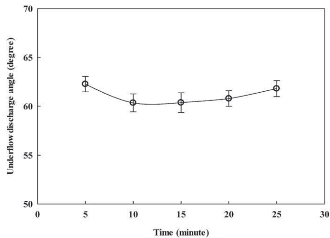
Fig. 3. Variation of spray angle at different time intervals at a fixed operating condition (standard deviations are indicated by vertical error bars).
