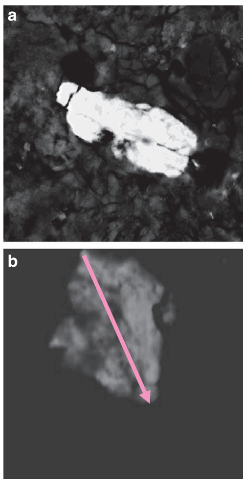
Fig. 3 Observation of Pb-phosphates in pea rhizosphere by SEM image and EDS analysis. a for soluble \text{KH}_2\text{PO}_4 amendment, \text{Pb}_5(\text{PO}_4)_3(\text{OH})_2 (Hydroxypyromorphite) was observed. b for solid hydroxyapatite, the following Pb-Ca-P associations were observed: (1) \text{Ca}_{4.5}\text{Pb}_{0.5}(\text{PO}_4)_3\text{OH} , (2) \text{Ca}_{4.0}\text{Pb}_{0.9}(\text{PO}_4)_3\text{OH} , (3) \text{Ca}_{3.3}\text{Pb}_{1.7}(\text{PO}_4)_3\text{OH} , and (4) \text{Ca}_{3.0}\text{Pb}_{2.0}(\text{PO}_4)_3\text{OH}
