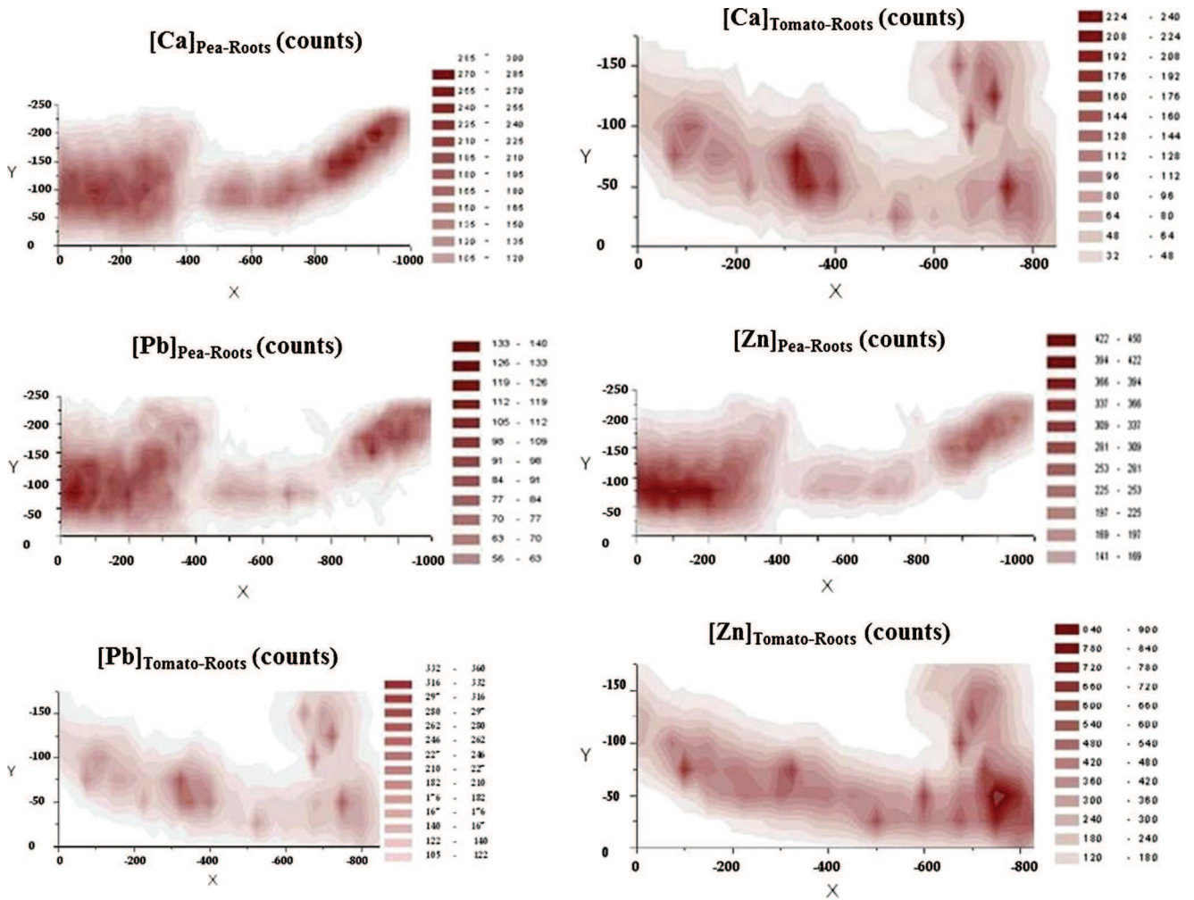
Fig. 2 Spatial distribution of Pb and Zn in the root systems of pea and tomato determined by \mu FX after plant cultures on the polluted soil amended with \text{KH}_2\text{PO}_4
