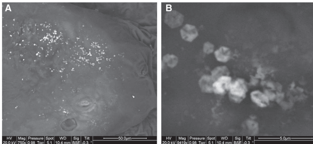
Fig. 4. BSE images of a necrotic area identified on lettuce leaf containing hexagonal \text{PbCO}_3 particles (a); Detailed view of \text{PbCO}_3 crystals (b).
