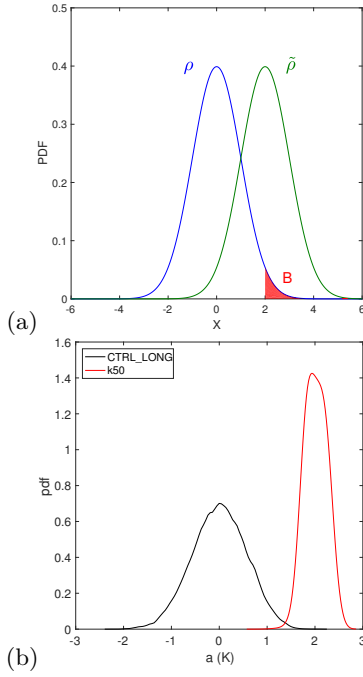
Fig. 3. (a) We want to estimate the probability to be in the set B , for the model PDF \rho(x) . We are able to sample rather from the PDF \tilde{\rho}(x) for which the rare event becomes common. We know the relation L = \rho/\tilde{\rho} and can recover the model statistics \rho , from the importance sampling \tilde{\rho} . (b) PDF of the time average temperature a ( T = 90 d) for the model control run (black) and for the algorithm statistics with k = 50 , illustrating the algorithm perform importance sampling and that +2^\circ K heat waves become common for the algorithm while they are rare for the model.
