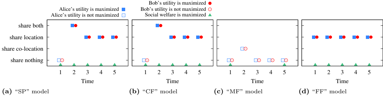
Fig. 2. Players' decisions at equilibrium, (s_{Alice}^*(t), s_{Bob}^*(t)) , for f_{sv} = 0.57 , f_{lc} = 0.56 , f_{pb} = 0.60 and different adversarial models: (a) Service Provider (SP), (b) Our friends in common (CF), (c) My other friends (MF), (d) My friend's other friends (FF) models.
