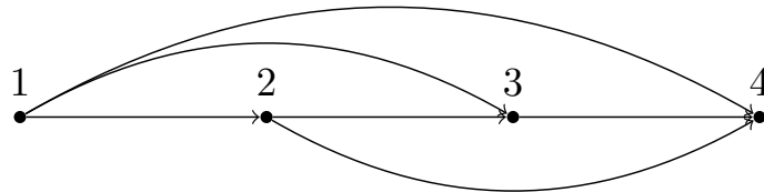
Figure 13: Example of an auxiliary graph.
