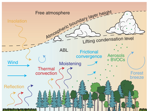
Figure 4 | Possible pathways of temperate forest impact on convective cloud formation.
