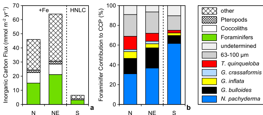
Fig. 3. (a) Varying annual inorganic carbon ( \text{CaCO}_3 ) fluxes in iron fertilized (+ Fe) and low-iron (HNLC) waters according to sediment trap data from north (N), northeast (NE), and south (S) of Crozet Plateau in the southern Indian Ocean (Salter et al., 2014). Planktic foraminifer tests and shell fragments contribute most of the compound specific particles, followed by coccoliths and pteropods. 'Other' inorganic carbon flux may include fragments of larger organisms, and coccolith within fecal pellets. (b) Near Crozet, N. pachyderma is a major contributor to the species-specific shell calcite production and carbonate counter pump (CCP). Planktic foraminifer tests of the 63–100 \mu\text{m} size-fraction are not classified. Absolute and relative fluxes of planktic foraminifers, coccolithophores, and pteropods may vary even stronger on a larger regional scale than between the + Fe and HNLC water around Crozet Plateau (Salter et al., 2014, Rembauville et al., 2016a).
