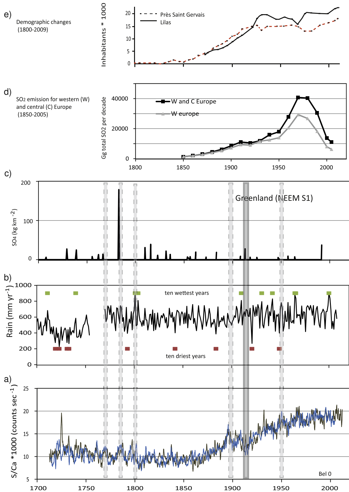
Fig. 4. Comparison between S/Ca * 1000 evolution through time for Bel 0 speleothem (a) with other environmental parameters, precipitations recorded in Paris, after Slonosky, 2002 (b), Volcanic SO 4 emissions as reconstructed by Greenland ice cores (Sigl et al., 2013) (c), SO 2 emissions (in Gg per decade), after Smith et al., 2011 (d), demographic evolution, data from Motte et al., 2003 (e). Light and dotted shades are the positives peaks observed within the two samples (only Bel 0 is presented here) and the dark one is the negative peak also repeated within the two samples.
