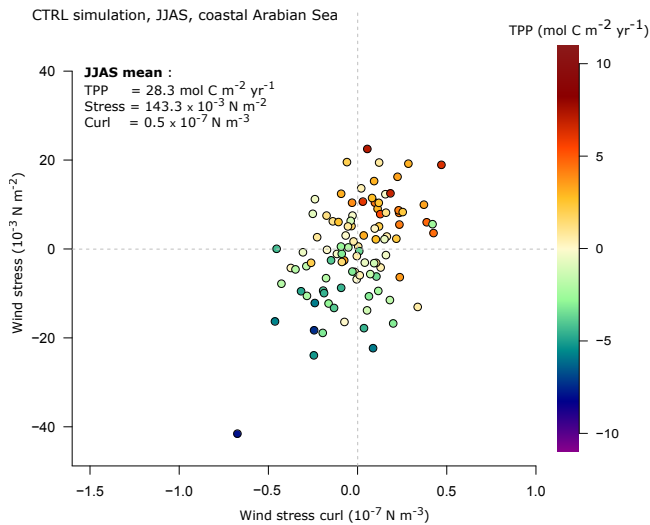
Figure 4. Anomalies of total primary productivity (TPP, \text{mol C m}^{-2} \text{yr}^{-1} , represented by the colour scale) integrated over the whole water column as a function of wind stress anomalies ( 10^{-3} \text{ N m}^{-2} , y axis) and wind stress curl anomalies ( 10^{-7} \text{ N m}^{-3} , x axis) in the western coastal Arabian Sea (see Fig. 2a) for the CTRL simulation. Anomalies are computed as the difference between each summer average (JJAS) and the seasonal summer mean of the corresponding variable in the CTRL simulation. The colour of the circles represents the value of the change in TPP compared with the CTRL. The colour scale, x axis range and y axis range are the same as those in Figs. 7 and 10.
