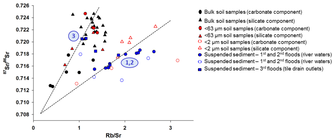
447 Figure 7. ^{87}\text{Sr}/^{86}\text{Sr} vs Rb/Sr in suspended sediment, carbonate and silicate soil samples (<2 mm, <63 \mu\text{m} and <2 \mu\text{m} fractions). 1,2,3: 448 suspended sediment sampling campaign number. 449
