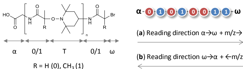
Scheme 1. Molecular structure and nomenclature of the sequence-coded oligo(alkoxyamine amide)s studied in the present work.
