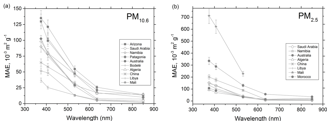
Figure 3. Spectral dependence of the MAE values for the samples investigated in this study in the PM 10.6 (a) and in the PM 2.5 (b) mass fractions.
