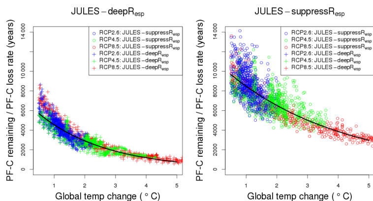
Figure 11. The permafrost carbon remaining in any given year divided by the loss of permafrost carbon in that year (FCRt) as a function of global mean temperature change ( \Delta T ). The black line is the exponential fit to the model points.
