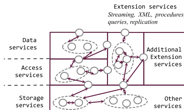
Fig. 7 Service-oriented DBMS [101]
