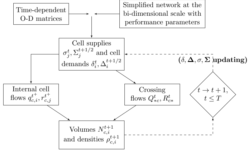
Fig. 2: Bi-dimensional network flows computing engine.
