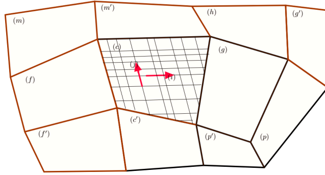
Fig. 1: Surface of the large-network (as the network-domain) is dis-aggregated in 2d -zones. Zones are meshed in quadrangular cells. Each cell has certain parameters: a finite number of preferred propagation directions of flows, numbers of lanes in each direction, lengths of lanes in each direction.
