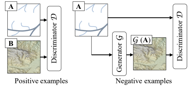
Fig. 4. Overview of the training of a cGAN: The discriminator \mathcal{D} learns to classify between real and synthesized pairs, whereas the generator \mathcal{G} learns to fool the discriminator.
