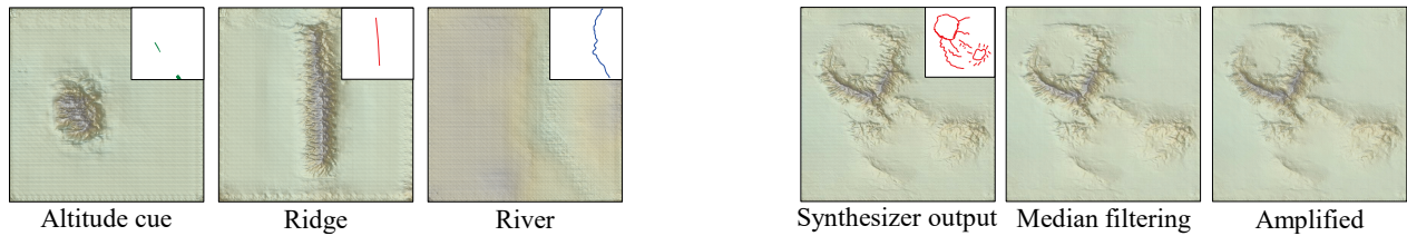
Fig. 25. Failure case: sometimes when the input sketch is too sparse, our method generates repeated terrain patches and grid artifacts.
