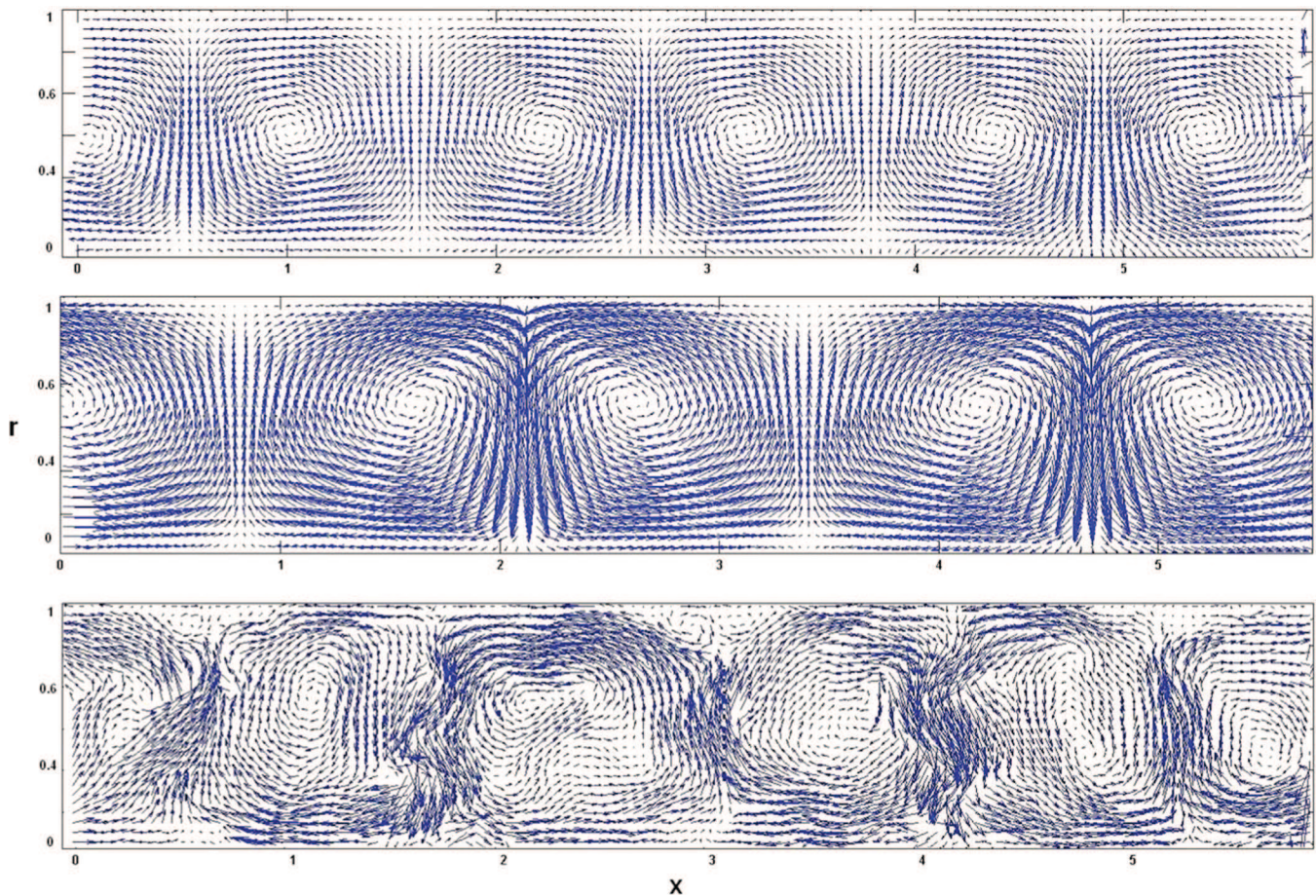
Fig. 5. Instantaneous velocity fields in the (r-x) -plane measured by PIV ( \eta = 0.687 ). From top to bottom: Re=80 (TVF), Re=636 (WVF), and Re=6000 (TTVF).
