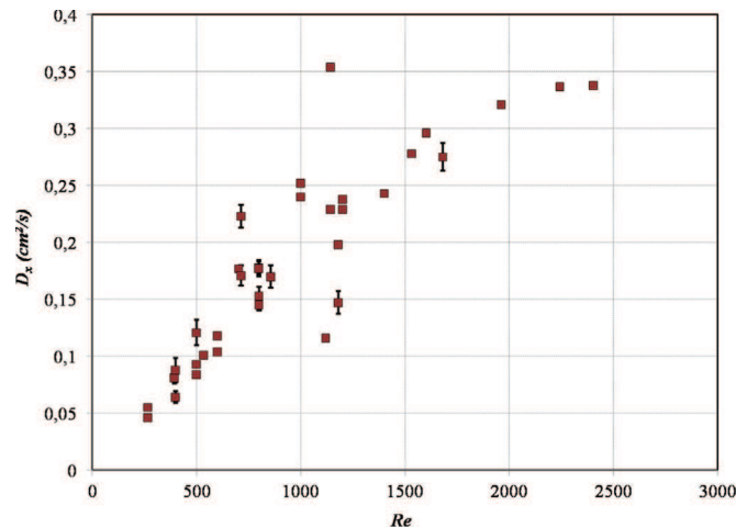
Fig. 10. Dispersion coefficient D_x as a function of Re ( \eta = 0.85 ).
