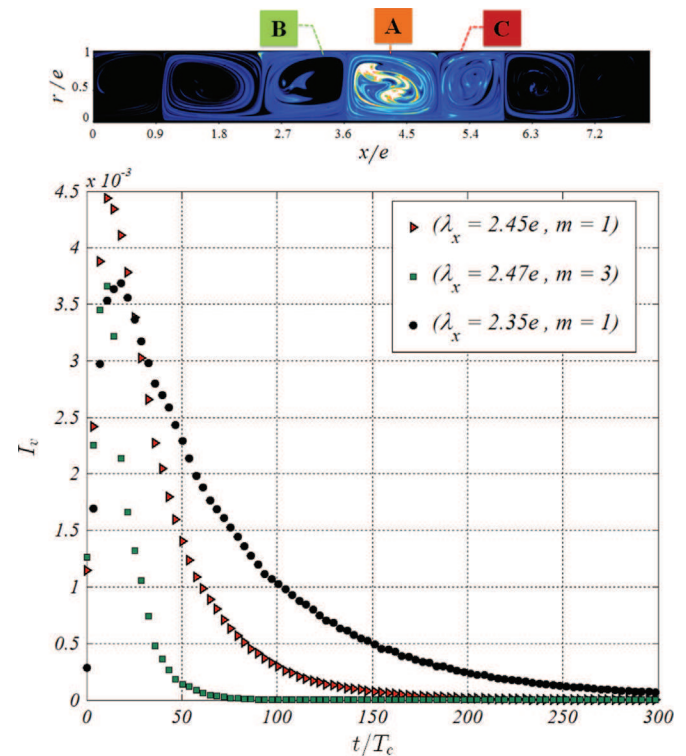
Fig. 11. Intervortex mixing between vortex A and B (outflow zone), influence of the wave state ( Re=1082 ) - T_c = 0.9 s is the rotation period of the inner cylinder.
