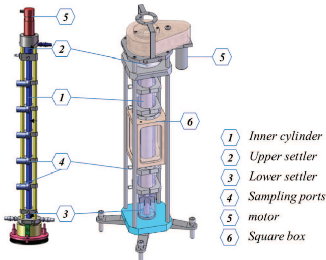
Fig. 1. Schematic presentation of the apparatus: Left: 1 st prototype ( \eta=0.85 ) – Right: 2 nd prototype ( \eta=0.687 ).
