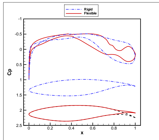
Figure 5: Shapes and distributions of C_p at 40 kts BS for the rigid and flexible hydrofoils.
