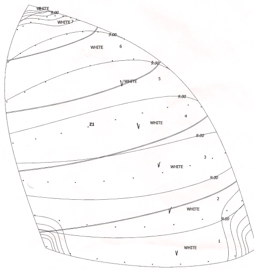
(b) Illustration of cross-cut panelling
