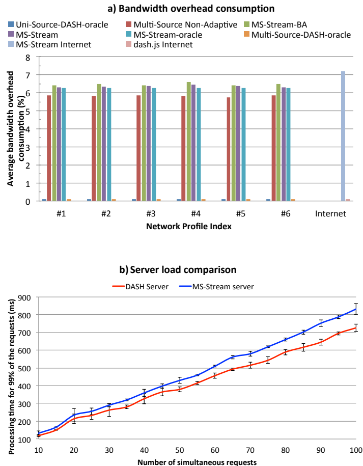
Figure 6: Overhead evaluation
