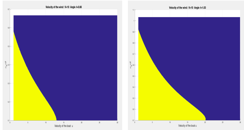
Figure 5b. The speed can be greater than 2V .
