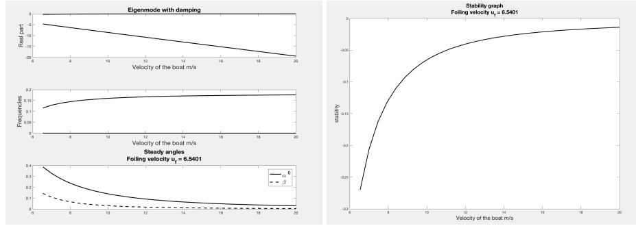
FIGURE 18. The spectrum (left) and criterium of stability (right) for a = 0.2 and h = 5 .
