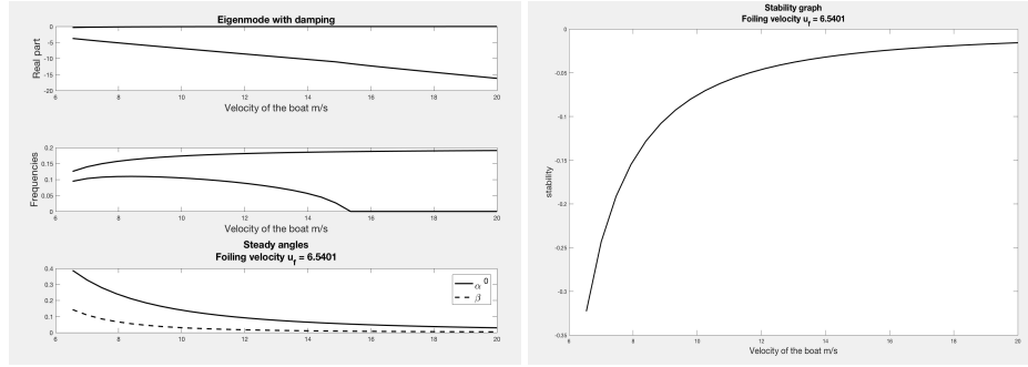
FIGURE 17. The spectrum (left) and criterium of stability (right) for a = 1 and h = 5
