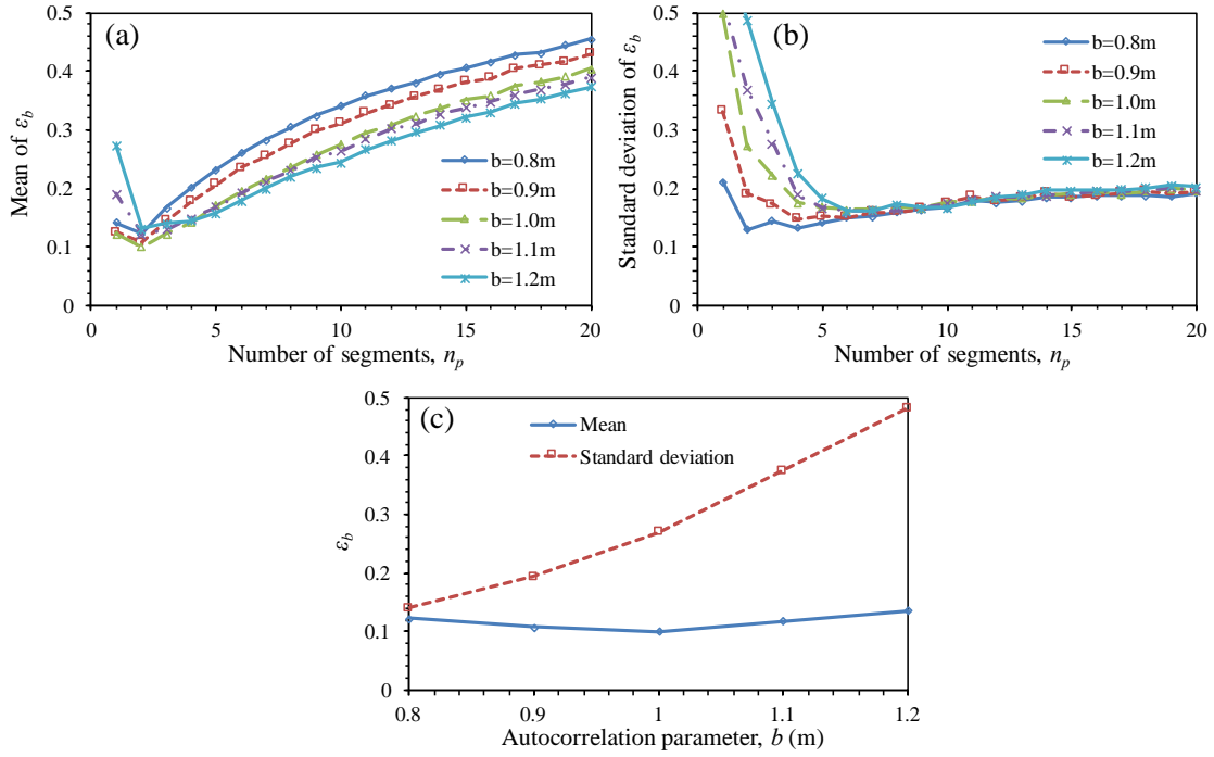
Figure 5. Sensitivity of \varepsilon_b for: (a) the mean of \varepsilon_b , (b) the standard deviation of \varepsilon_b , and (c) the mean and standard deviation of \varepsilon_b for n_p=2 ( N_s=200 , L=100 m).
