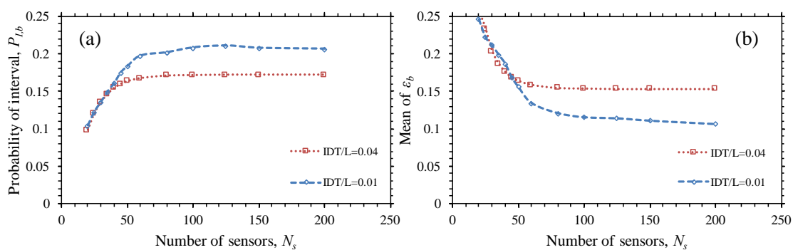
Figure 10. Effect of N_s on (a) the probability of interval P_{L,b} , and (b) the mean of \epsilon_b , for \Delta=10\% and n_p optimized.
