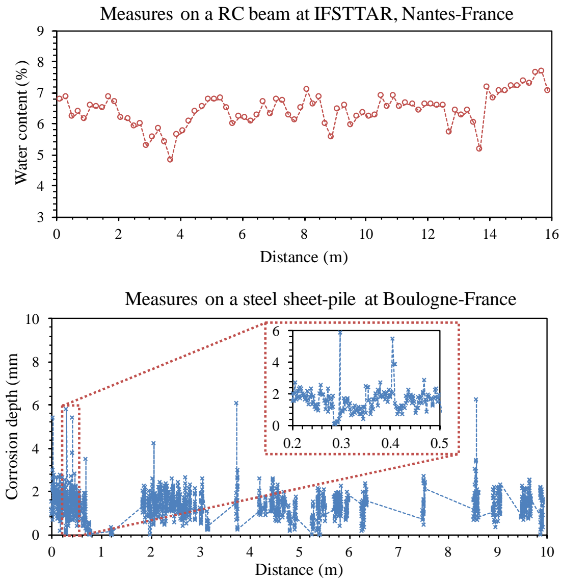
Figure 11. Experimental trajectories of water content (up) and corrosion (down).
