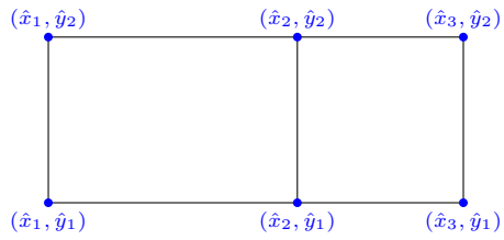
Figure 5: Physical domain \Omega
