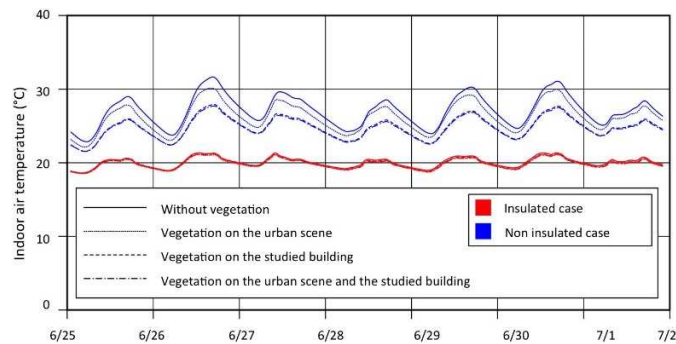
Figure 7. Indoor air temperatures (average of all five floors) for the insulated and non-insulated cases.
