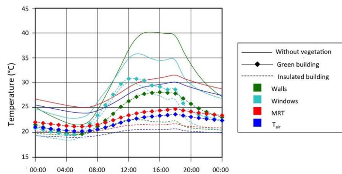
Figure 11. Internal surface temperature of windows and walls, mean radiant temperature (MRT) and indoor air temperature ( T_{\text{air}} ) of the third floor on 26 June 2010.
