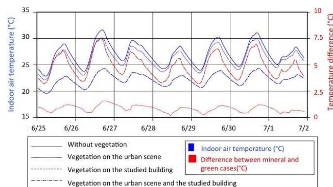
Figure 8. Indoor temperatures of the third floor (in blue) and the difference with the mineral case (in red). Nota bene (N.B.): the results of the cases “vegetation on the studied building” and “vegetation both in the urban environment and on the studied building” are superimposed.
