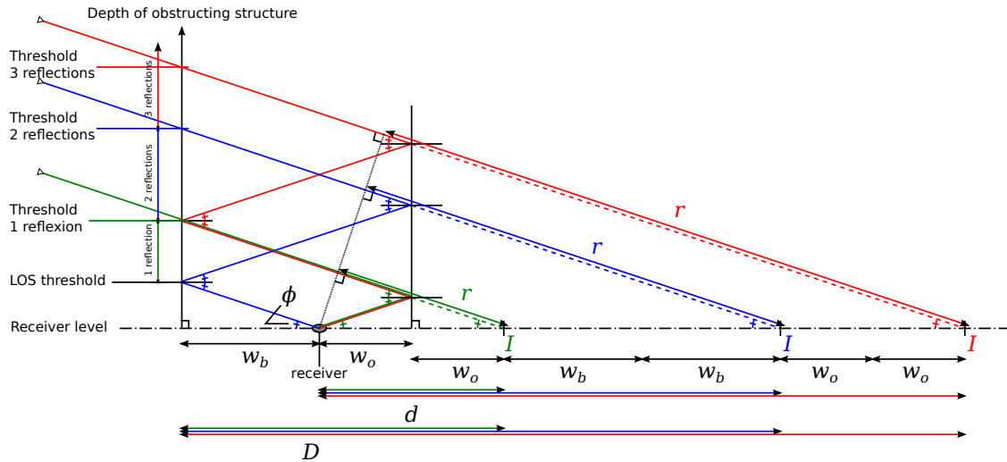
Figure 16. Reflected GNSS rays trajectories following the cross-section in the plane defined by the ray and receiver.
