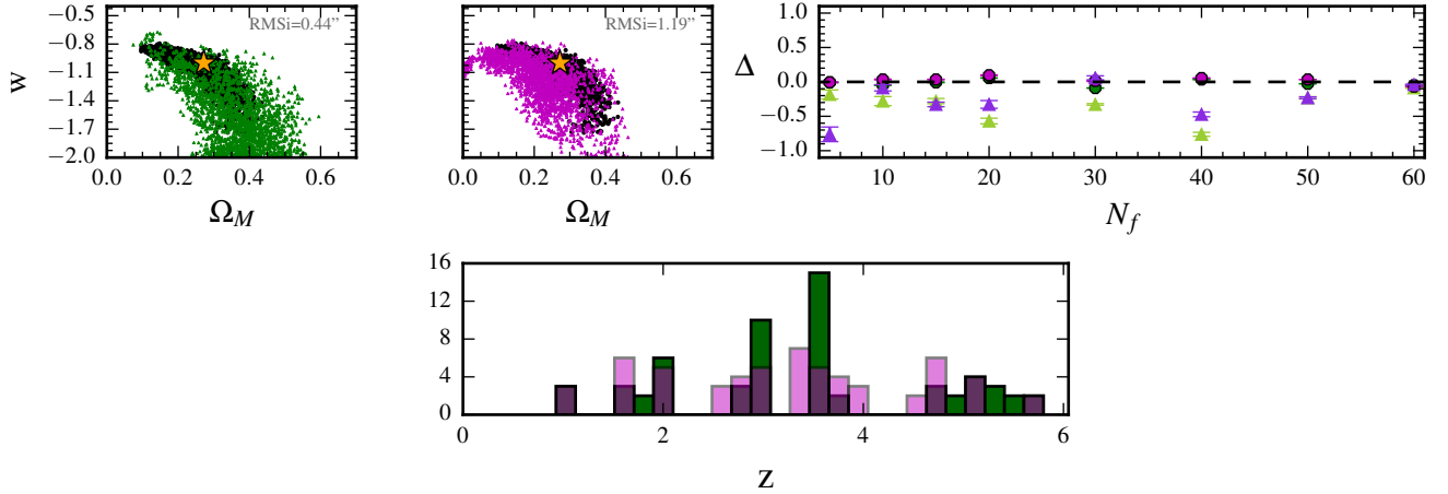
Figure 9. Top left and middle panels: constraints on the \Omega_M and w parameters for Ares for the model NFW - HERNQUIST. As filled black circles, the fiducial constraints (all multiple images with spectroscopic redshifts); as green and magenta filled triangles are plotted the constraints from two models with a (slightly different) reduced catalogue of spectroscopic redshifts (shown in the bottom panel). Right panel: systematic bias in the recovery of cosmological parameters as a function of increasing photometric families added in the modelling (with a 0.04(1+z) precision). The filled triangles show the bias on the w parameter and the filled circles, on the \Omega_M parameter. The statistical error is represented by the error bars.
