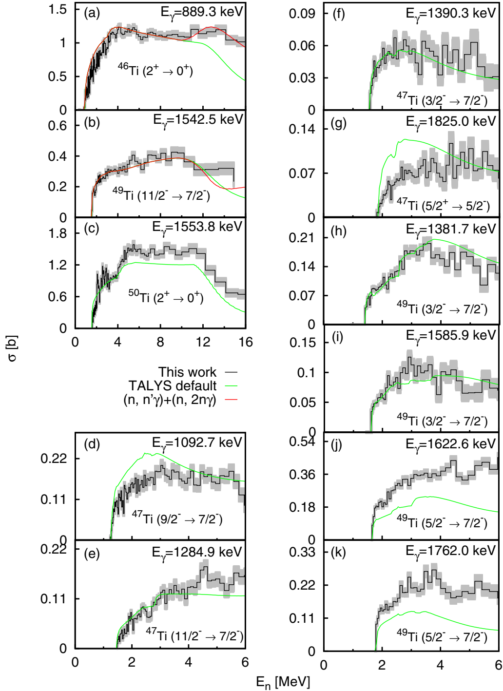
FIG. 7. The production cross sections of the \gamma rays observed from the minor isotopes of ^{nat}\text{Ti} in comparison with TALYS theoretical calculations performed using the default input parameters. The total absolute uncertainties of our experimental values are displayed in gray.
