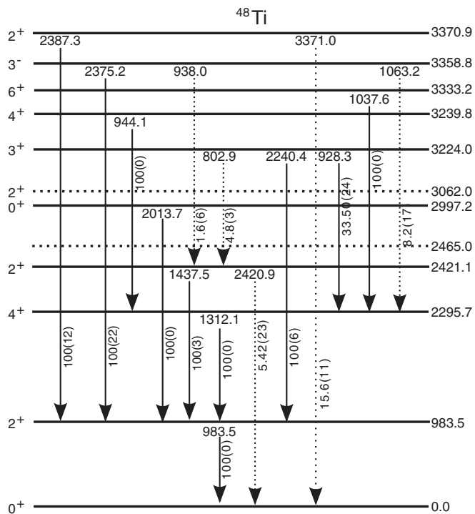
FIG. 1. Simplified level scheme of the ^{48}\text{Ti} nucleus [39]. The observed transitions are displayed using solid lines. The dashed line is used to show known transitions that were not observed but were taken into account in the data analysis procedure or to display the levels with no or unknown \gamma -ray contribution.
