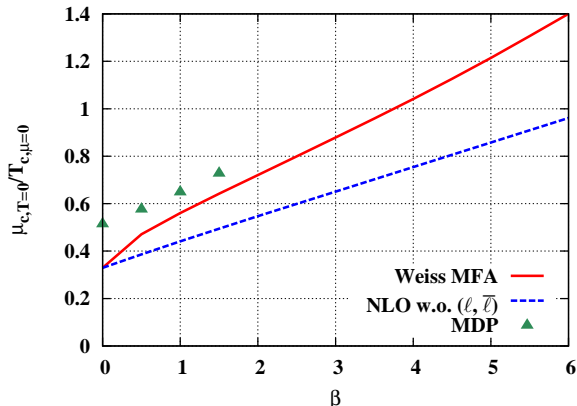
FIG. 13: (Color online) The ratio R = \mu_{c,T=0}/T_{c,\mu=0} as a function of the lattice bare coupling \beta = 2N_c/g^2 . For a comparison, we show the MDP results for R in Ref. [31]: We read off the \mu_{c,T=0} \simeq 0.72 from Fig. 6 in Ref. [31], and quoted the T_c(\beta) evaluated by using the “exponential extrapolation” to calculate the R .
