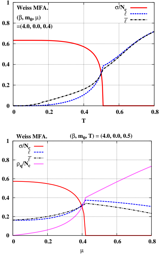
FIG. 6: (Color online) Upper: The chiral condensates \sigma , Polyakov loops ( \ell, \bar{\ell} ), in NLO Weiss MFA as a function of T at (\beta, m_0, \mu) = (4.0, 0.0, 0.4) in lattice units. Lower: The chiral condensates \sigma , Polyakov loops ( \ell, \bar{\ell} ), and quark number density \rho_q/N_c in NLO Weiss MFA as a function of \mu at (\beta, m_0, T) = (4.0, 0.0, 0.5) in lattice units.
