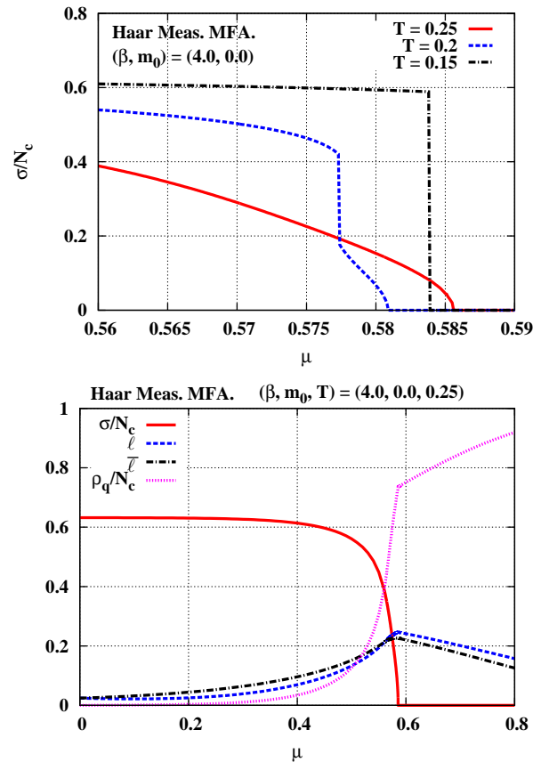
FIG. 3: (Color online) Upper: The chiral condensates \sigma , Polyakov loops ( \ell, \bar{\ell} ), in NLO Haar measure MFA as a function of \mu at (\beta, m_0) = (4.0, 0.0) for the selected temperatures T = 0.15, 0.2, 0.25 in lattice units. Lower: The \sigma , ( \ell, \bar{\ell} ), and quark number density \rho_q in NLO Haar measure MFA as a function of \mu at (\beta, m_0, T) = (4.0, 0.0, 0.25) in lattice units.
