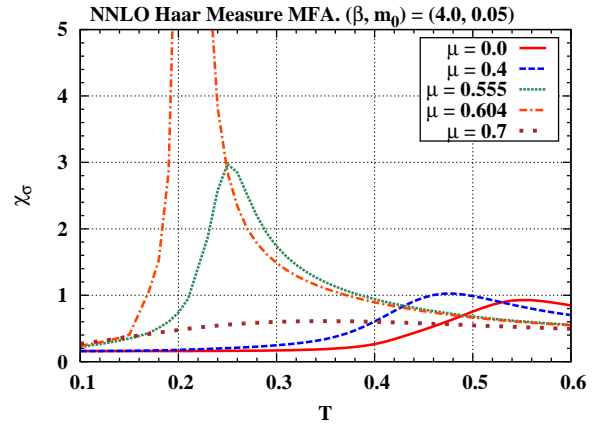
FIG. 15: (Color online) The chiral susceptibility in NNLO Haar measure MFA with m_0 = 0.05 as a function of temperature for various \mu . All quantities are in lattice units at the coupling \beta = 4.0 .
