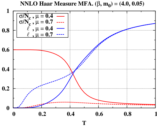
FIG. 14: (Color online) Chiral condensates and Polyakov loops in the NNLO Haar measure MFA for \beta = 4.0 with m_0 = 0.05 as a function of temperature at the two chemical potentials \mu = 0.4 and 0.7 . All quantities are in lattice units.
