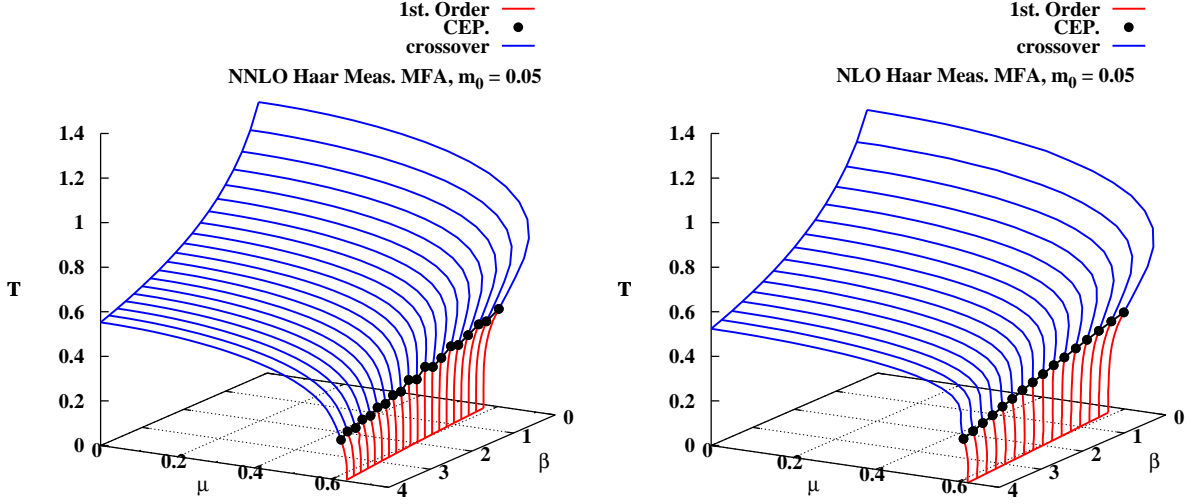
FIG. 17: (Color online) The phase diagram evolution for m_0 = 0.05 as a function of \beta in NNLO Haar-measure MFA (left), which is compared with the counterpart in NLO Haar-measure MFA (right) with same parameters. The red and blue lines represent the first-order chiral transition and the chiral crossover, respectively. The black points show the CEP separating the first-order and crossover phase boundaries. The little fluctuations of the CEP in the NNLO case are due to limited precision in the numerical search of the maximum of chiral susceptibilities as a function of T and \mu . All quantities are in lattice units at a given \beta .
