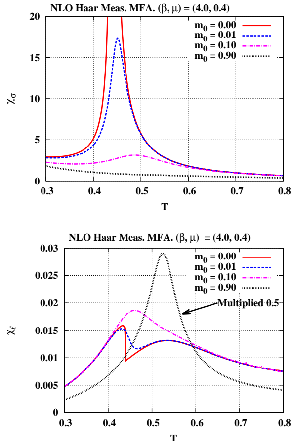
FIG. 10: (Color online) The chiral (upper) and Polyakov loop (lower) susceptibilities as a function of T for various bare quark mass m_0 at (\beta, \mu) = (4.0, 0.4) in NLO Haar measure MFA. All quantities are in lattice units.
