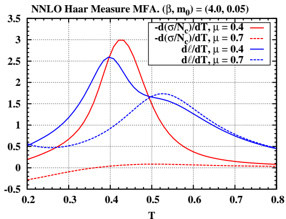
FIG. 16: (Color online) The temperature derivative of the chiral condensates and Polyakov loops in the NNLO Haar measure MFA with m_0 = 0.05 as a function of temperature at \mu = 0.4 and 0.7 . All quantities are in lattice units at the coupling \beta = 4.0 .
