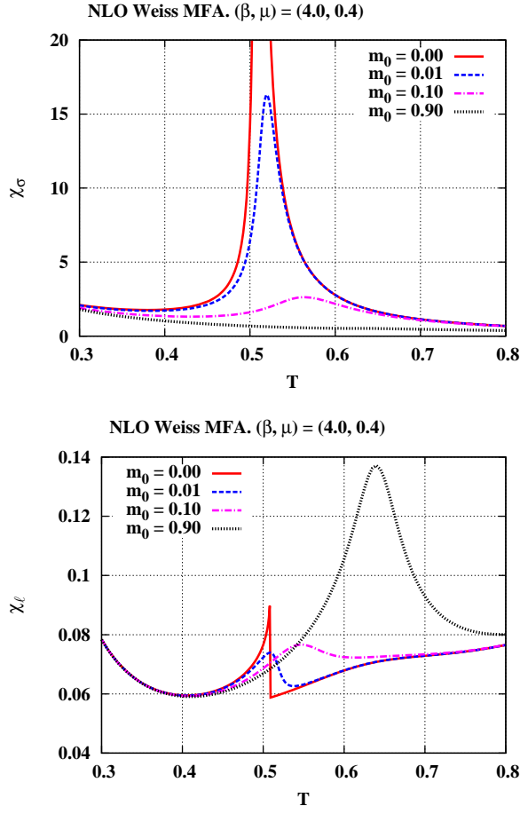
FIG. 11: (Color online) The chiral (upper) and Polyakov loop (lower) susceptibilities as a function of T for various bare quark mass m_0 at (\beta, \mu) = (4.0, 0.4) in NLO Weiss MFA. All quantities are in lattice units.
