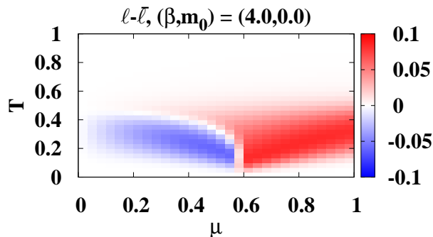
FIG. 5: (Color online) Upper: The phase diagram of NLO Haar measure MFA at (\beta, m_0) = (4.0, 0.0) in lattice units. See texts for details. Lower: The difference of the Polyakov loop and anti-Polyakov loop in the phase diagram of the NLO Haar measure MFA.
