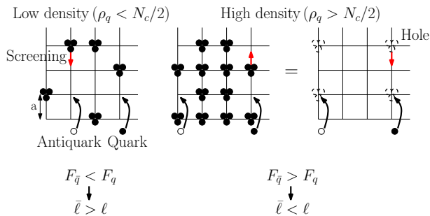
FIG. 4: (Color online) The half-filled and saturation.
