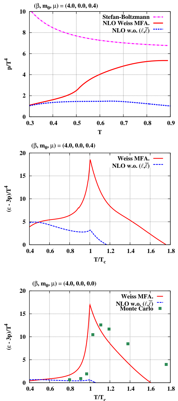
FIG. 9: (Color online) The pressure (upper) and interaction measure (middle and lower) normalized by T^4 in “NLO Weiss MFA” and “NLO without Polyakov loops” as a function of T at (\beta, m_0, \mu) = (4.0, 0.0, 0.4) (upper and middle), and (\beta, m_0, \mu) = (4.0, 0.0, 0.0) (lower). In the upper panel, the horizontal axis T is in lattice units. In the middle and lower panels, the horizontal axis is normalized by critical temperature T_c . In the lower panel, we have quoted the Monte Carlo results [40].
