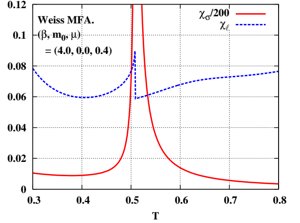
FIG. 7: (Color online) The chiral and Polyakov loop susceptibilities ( \chi_\sigma, \chi_\ell ) in NLO Weiss MFA as a function of T at (\beta, m_0, \mu) = (4.0, 0.0, 0.4) in lattice units. For a comparison, the chiral susceptibility \chi_\sigma has been multiplied by 1/200.
