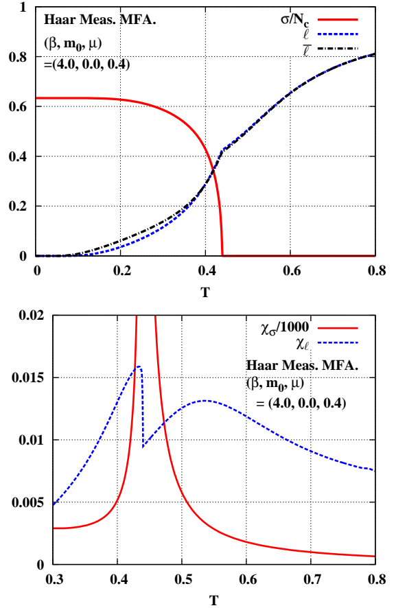
FIG. 2: (Color online) Upper: The chiral condensates \sigma , Polyakov loops ( \ell, \bar{\ell} ), in NLO Haar measure MFA as a function of T at (\beta, m_0, \mu) = (4.0, 0.0, 0.4) in lattice units. Lower: The chiral and Polyakov loop susceptibilities ( \chi_\sigma and \chi_\ell ) in the same condition as the upper panel in lattice units. For a comparison, the \chi_\sigma is multiplied by 1/1000.
