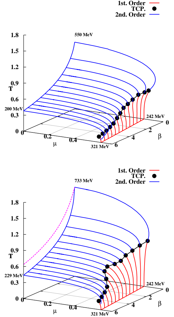
FIG. 12: (Color online) The phase diagram evolution with the increasing lattice coupling \beta at NLO Haar measure (upper) and Weiss (lower) MFA in the chiral limit. We have quoted a^{-1}(\beta = 0) = 440 (MeV) and a^{-1}(\beta = 6) = 524 (MeV) from Ref. [45]. In Weiss MFA (lower), we have also shown our previous result on the transition temperature at \mu = 0 without effects of plaquette-driven Polyakov loops [25] by the magenta-dashed line.
