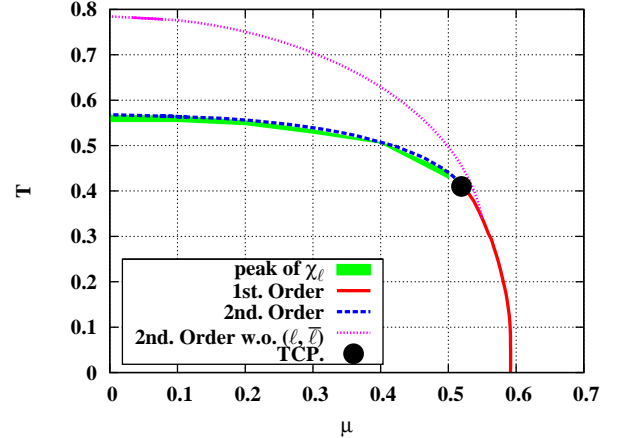
FIG. 8: (Color online) The phase diagram at (\beta, m_0) = (4.0, 0.0) in NLO with Weiss MFA in lattice units. See texts for details.
