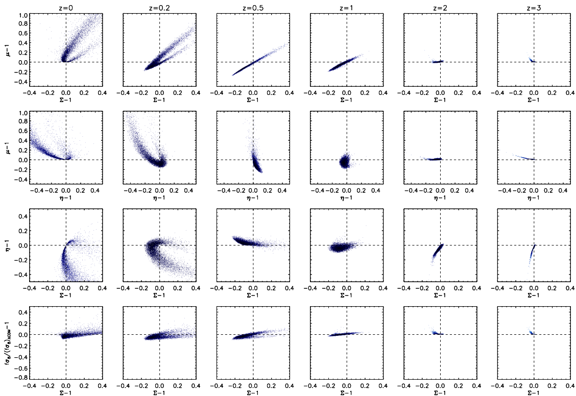
Figure 1: The correlations between \mu , \eta , \Sigma and f\sigma_8 is displayed at several redshift epochs, from left to right z = 0, 0.2, 0.5, 1, 2, 3 , for 10^4 EFT models in the LDE scenario. The background evolution has been set to match that of a flat \Lambda\text{CDM} model. The \Lambda\text{CDM} prediction corresponds to the intersection of the two dashed lines. The gray scale highlights the density of points.
