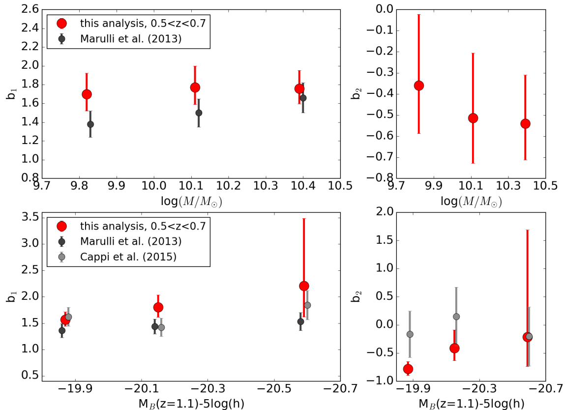
Fig. 9. Galaxy linear bias (left panels, b_1 ) and non linear bias (right panels, b_2 ) as a function of stellar mass (upper panel) and luminosity (lower panel). Independent measurements obtained on the same subsamples are shown for comparison: from the 2PCF (black points Marulli et al. 2013) and from volume-averaged higher-order correlation functions (grey points Cappi et al. 2015). The values on the x-axis have been slightly offset, for illustrative purposes.
