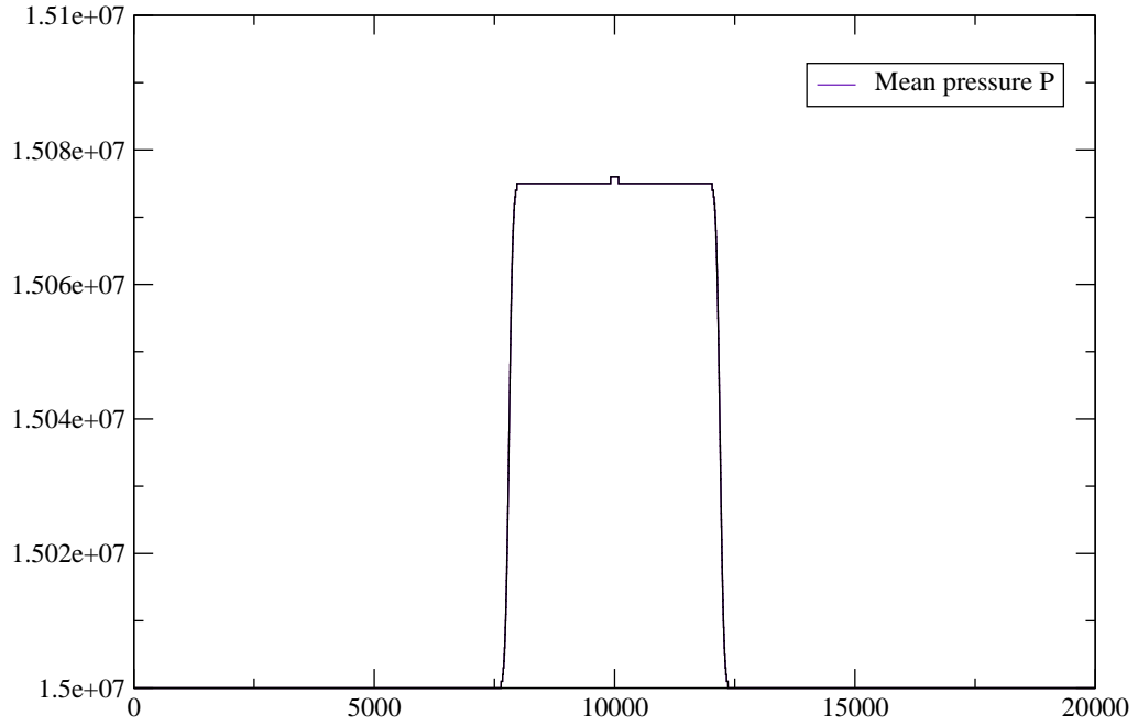
Figure 2. Standard three-fluid model - Mean pressure field P when the flow hits a wall boundary.
