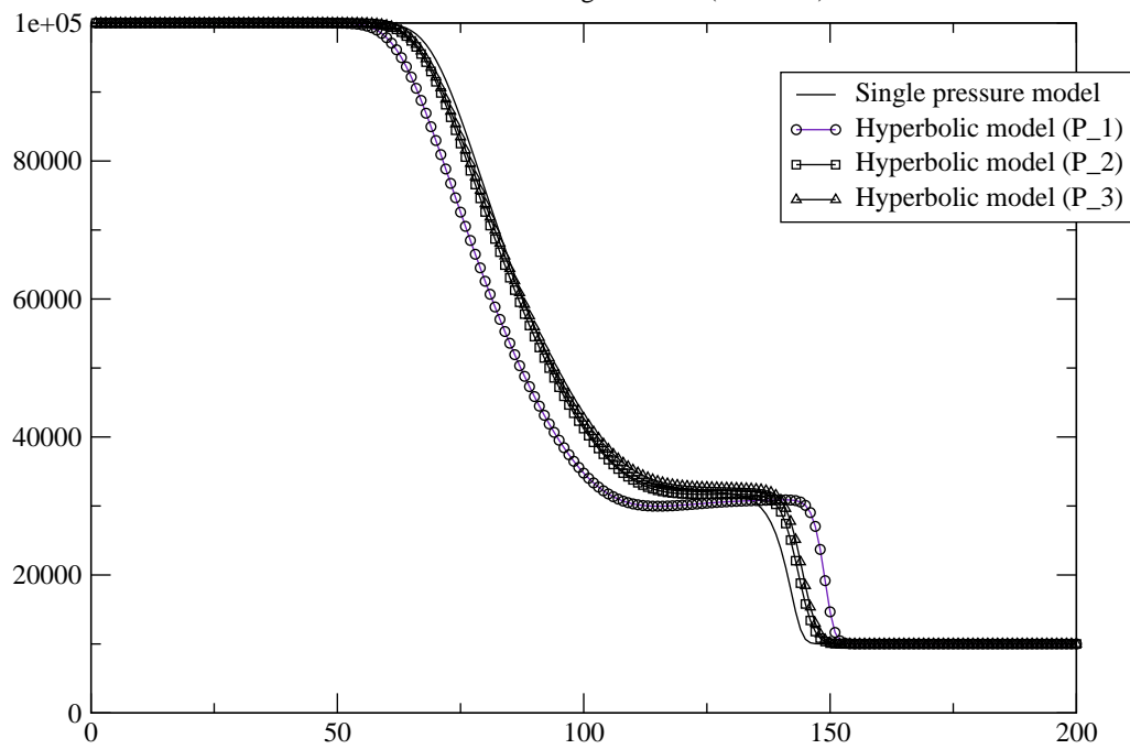
Figure 4. Shock tube experiment. Both approaches are compared using very large relaxation time scales for pressure and velocity fields.
