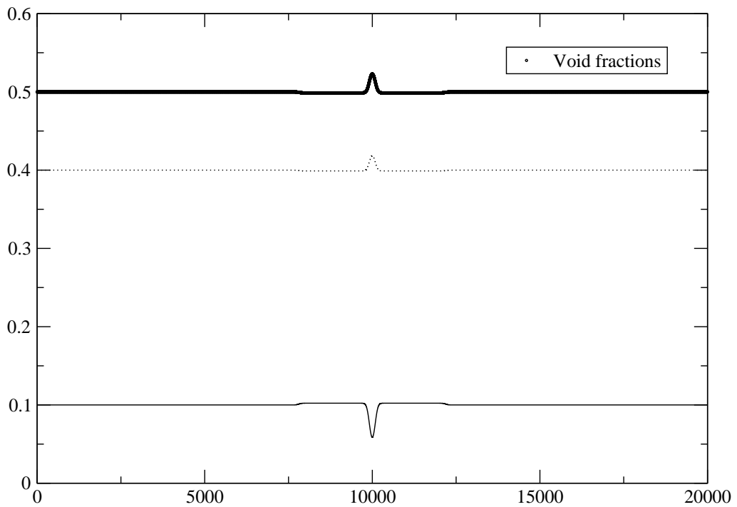
Figure 3. Standard three-fluid model - Void fraction distribution when the flow hits a wall boundary. \alpha_1 (plain line), \alpha_2 (dotted line), \alpha_3 (circles)
