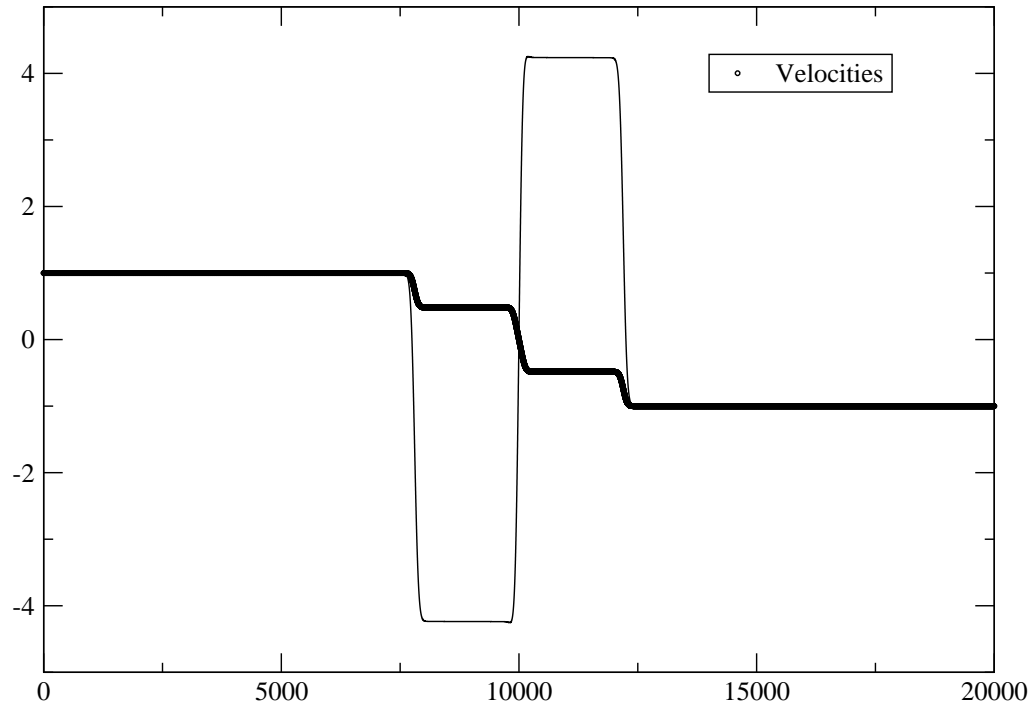
Figure 1. Standard three-fluid model - Velocity fields when the flow hits a wall boundary. U1 (plain line), U2 (dotted line), U3 (circles)
