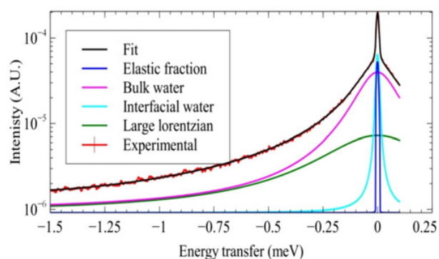
Figure 1. Experimental and calculated contributions for Q = 0.95 \text{ \AA}^{-1} on IN5.
