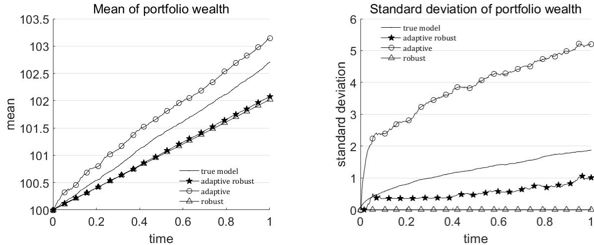
Figure 5: Time-series of portfolio wealth means, and standard deviations. Unknown mean and variance.
