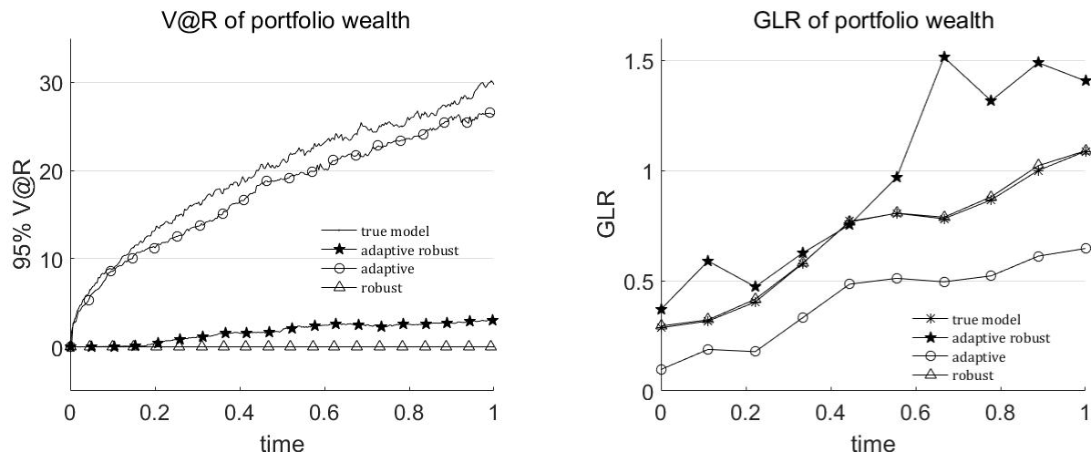
Figure 2: Time-series of portfolio V@R and GLR. Unknown mean.
