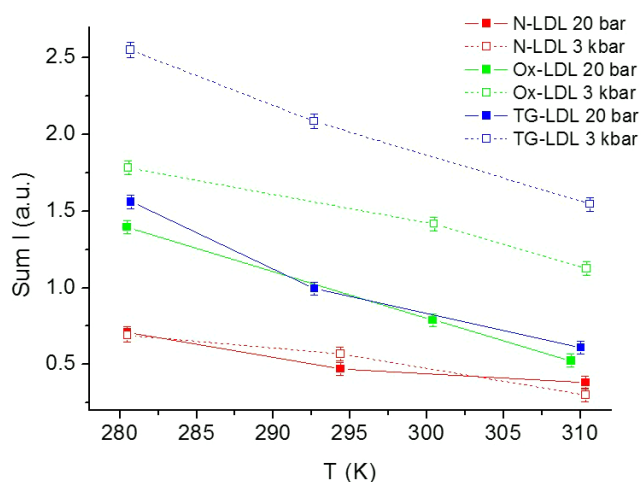
Fig. 2. Neutron intensities summed over all scattering angles as a function of temperature for both pressure points. Lines are guides to the eyes.
