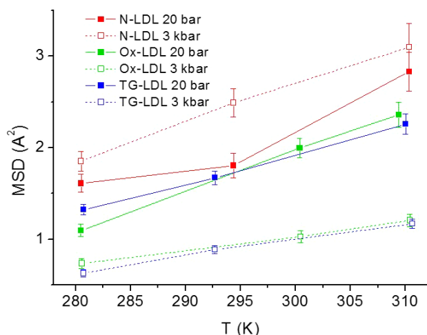
Fig. 3. Atomic MSD extracted in the Q -range between 0.5 \text{ \AA}^{-1} and 2.0 \text{ \AA}^{-1} as a function of temperature for both pressure points. Lines are guides to the eyes.
