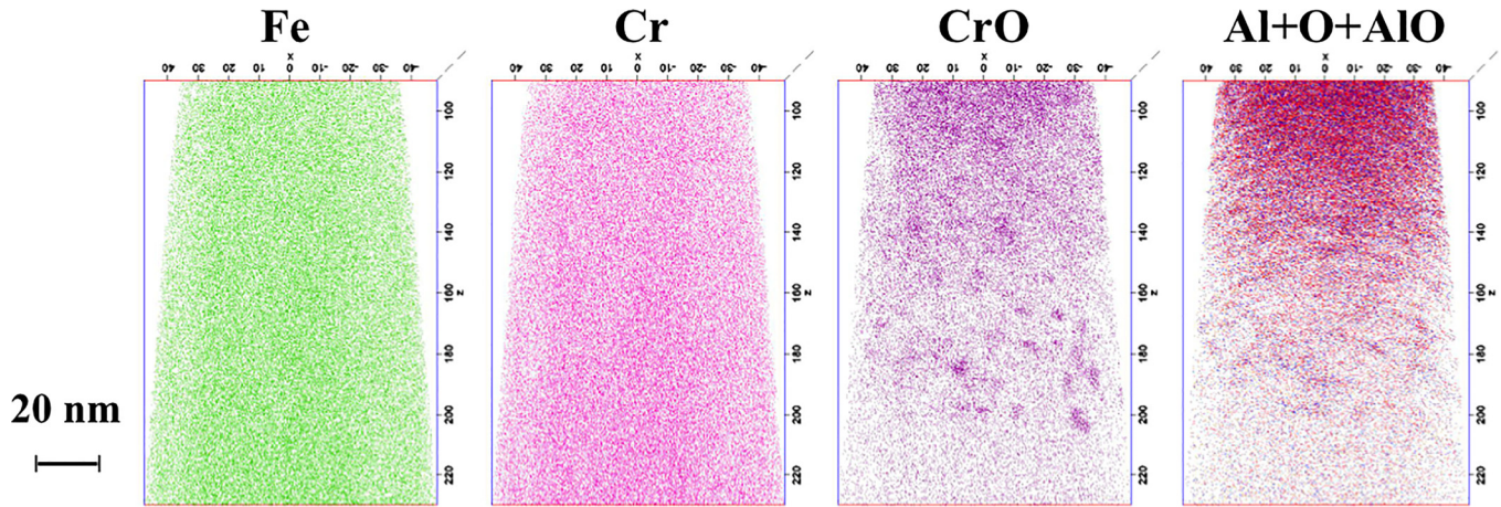
FIG. 17. 3D APT reconstruction from the annealed tip showing the distribution of evaporated elements and molecular fragments.
