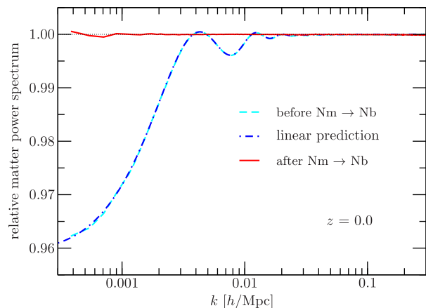
Figure 3. The cyan (dashed) line shows the matter power spectrum at redshift z = 0 of a Newtonian simulation that ignored radiation perturbations, relative to a simulation that included those perturbations in Nb gauge. As shown, this discrepancy is well described by a linear prediction computed in CLASS (blue, dot-dashed line). It can be accounted for by interpreting the result in terms of the Nm gauge. To demonstrate this, the red (solid) line shows the matter power spectrum after the particles have been displaced according to the gauge transformation that brings them from Nm gauge back to Nb gauge. The N -body simulations for this plot were performed with gevolution , and the linear transfer function for the gauge generator was provided through a modified version of CLASS.
