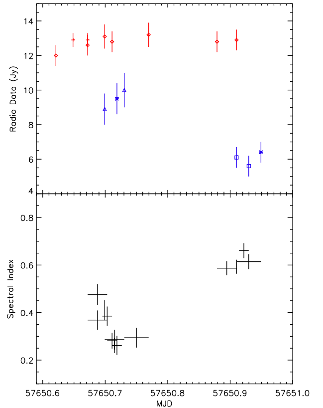
Figure 3. Zoom of the light curve and spectral index evolution presented in Fig. 2 during the maximum of the giant flare peak, on 2016 September 19.
