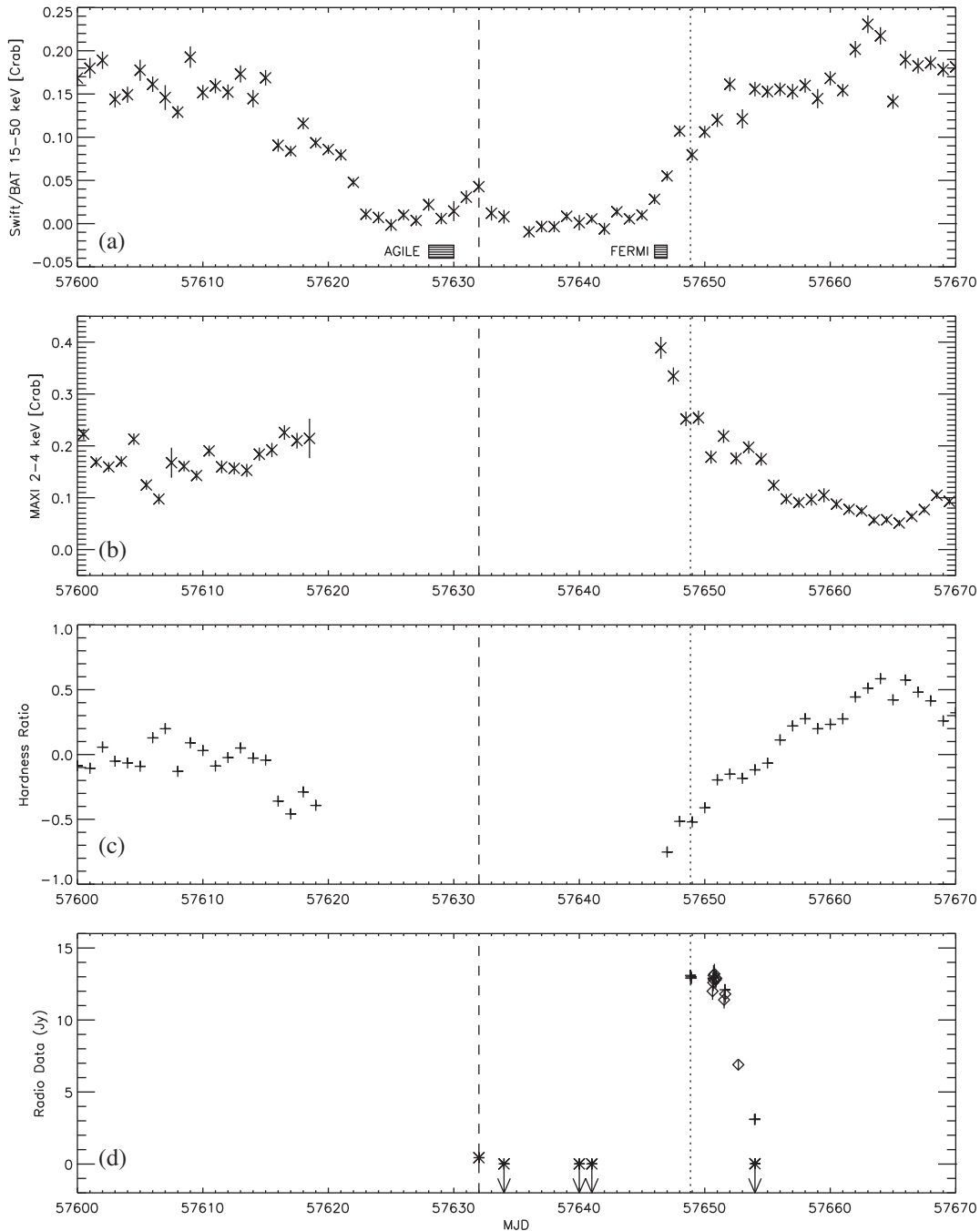
Figure 1. From the top to the bottom: (a) Swift /BAT 15–50 keV (Hard X-rays) light curve of Cyg X-3 in Crab units from 2016 July 31 to 2016 October 9. The gamma-ray detections with AGILE and Fermi /LAT are also reported; (b) MAXI 2–4 keV (Soft X-rays) light curve in Crab units; (c) hardness ratio corresponding to (Hard–Soft)/(Hard+Soft); (d) single-dish (cross: 8.5 GHz; diamond: 7.2 GHz) and VLBI data at 22 GHz (asterisk). The dashed line and the dotted line indicate the first VLBI observation and the first single-dish observation, respectively. The vertical arrows represent the VLBI upper limits at 5\sigma confidence.
