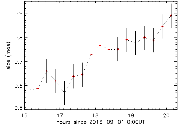
Figure 8. Radius in mas of the emitting component versus time corresponding to Fig. 7. The size increased within 4 h, which indicates a signature of the expansion of the emitting region.
