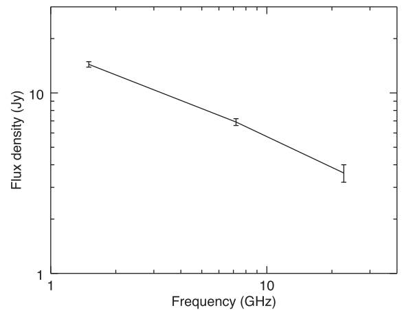
Figure 4. Optically thin spectrum obtained from SRT data at 1.5, 7.2 and 22.7 GHz 2 d after the maximum of the giant flare.
