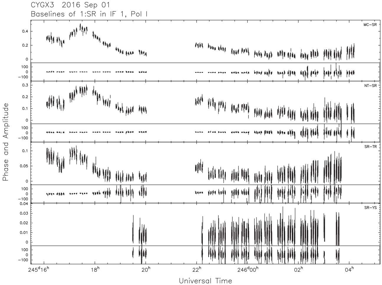
Figure 5. Cyg X-3 visibility amplitude and phase versus time for baselines to SRT for the 2016 September 1 (MJD 57632) observations at 22 GHz. Four pairs of panels are shown; from top to bottom: Sr-Mc, Sr-Nt, Sr-Tr, Sr-Ys; in each pair, the top panel shows amplitudes (in Jy) and the bottom phases (in degrees). Data are missing at around UT 21 for these baselines, due to SRT elevation limits (source transiting at zenith), but are in general present on other baselines. Note that the first part of the observation was missed by Yebes due to technical problems.
