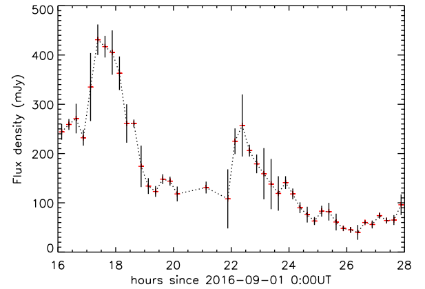
Figure 9. VLBI light curve obtained on 2016 September 1 (MJD 57632) showing a short-scale time variability, with the evidence of two peaks of different flux density during a mini-flare. The general trend of the off-peak measurements indicates a decrease of the flux during the observation.
