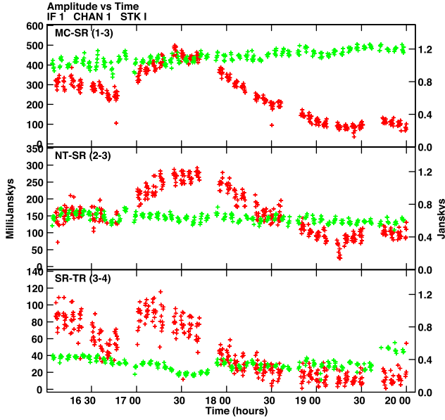
Figure 6. Visibility amplitudes of Cyg X-3 (red) and J2007+4029 (green) during the four first hours of the 2016 September 1 observation (MJD 57632). Variability is observed on the Mc-Sr, Nt-Sr, Sr-Tr baselines for Cyg X-3 within 2 h whereas the comparison source remains stable.
