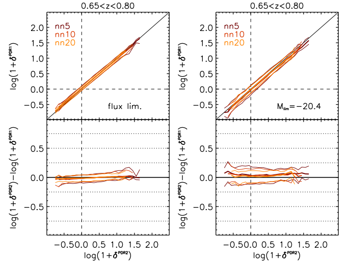
Fig. B.1. As in Fig. A.2, but here we compare the density field in the VIPERS PDR-1 sample and the density field used in this paper (for simplicity indicated as PDR-2 in the labels).
