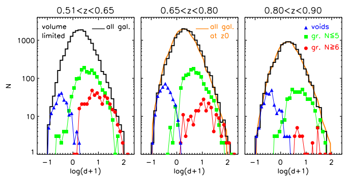
Fig. 2. Density distribution of the VIPERS galaxies in three redshift bins (three columns) for the entire sample (black histogram), for galaxies in voids (blue triangles), in groups with at most five members (green squares), and in groups with at least six members (red circles). See the text for the definition of groups and voids. The density field is computed with cylindrical filters, with a radius given by the fifth n.n. using the volume-limited tracers, which are complete up to z = 0.9 . To facilitate comparison, in the second and third redshift bins the orange line is the density distribution of the entire sample in the first redshift bin, normalised to the total number of galaxies in each bin.
