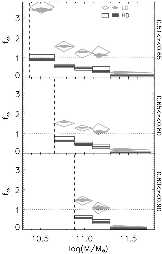
Fig. 6. Ratio of the number of active over passive galaxies ( f_{ap} ) in LD (light grey) and HD (dark grey) regions in the Rmocks (filled symbols) and in the Vmocks (empty symbols) in the same stellar mass bins and redshift ranges as in Fig. 5. In each mass bin, for the environment with fewer galaxies (HD for \log(M/M_{\odot}) < 11.29 , LD otherwise) we plot f_{ap} as computed directly from the mock catalogues, while for the environment with more galaxies we plot f_{ap} derived from the mass-matched samples. For not mass-matched values, symbols are centred on the y -axis on the mean value of f_{ap} of the 16 mock catalogues, and their height represents the rms around the mean. For mass-matched values, the y -axis position is computed as follows: first we compute the mean f_{ap} of the 100 mass-matched samples in each mock catalogue, then we average the 16 mean values. The height is given by the rms around this mean. For all symbols, the extension on the x -axis indicates the span of the stellar mass bin. For \log(M/M_{\odot}) > 11.29 , we show f_{ap} only for the Rmocks because the statistics in the Vmocks at these stellar masses is too low (see text). In each panel, the vertical and horizontal lines are the same as in Fig. 5.
