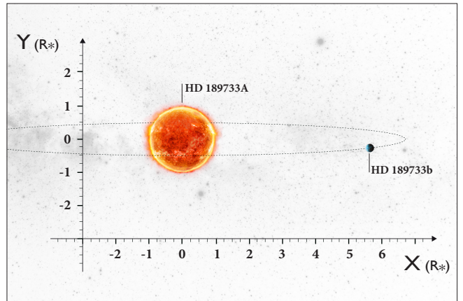
Figure 1. Artist representation of the exoplanet HD 189733b. HD 189733b orbits in nearly circular motion around its host-star HD 189733A; its orbital plane is parallel within about 4^{\circ} of the Earth-primary line of sight. Note the limb brightening effect emerging from the optically thin, stellar corona.
