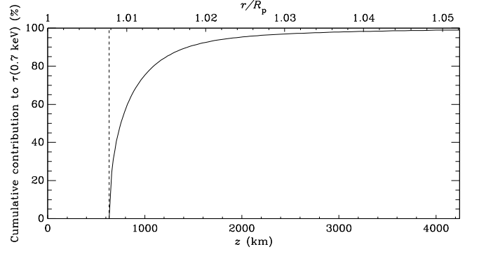
Figure 11. Cumulative contribution of the atmosphere at elevation z above the planetary radius to the optical depth at the X-ray absorption radius at 0.7 keV (vertical dashed line). The maximum elevation value on the x-axis corresponds to the atmospheric layer contributing for 99% to the optical depth.
