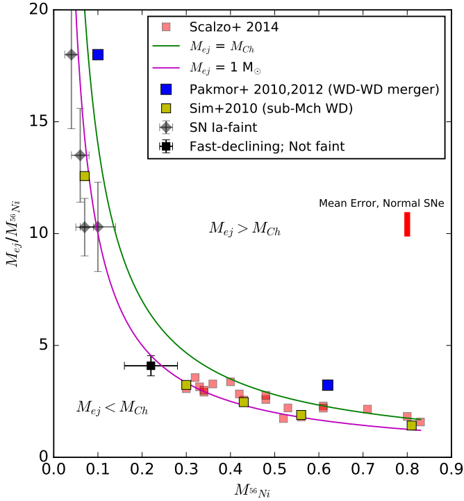
Fig. 3. Ratio of the ejecta mass to ^{56}\text{Ni} mass is plotted against the ^{56}\text{Ni} mass. With decreasing ejecta mass the black points are SNe 2005ke, 2006mr, 2007on 2007ax and 2009F, the last two of which lack NIR coverage. The diamonds are the SN Ia-faint sub-group and the square is 2007on which is fast-declining but not in the sub-group. The red points are normal SN Ia taken from Scalzo et al. (2014). We also plot the values from different model scenarios. The yellow squares are sub- M_{Ch} double detonation models from Sim et al. (2010), blue squares from violent merger models for normal and subluminous SNe from Pakmor et al. (2010, 2012), the green curve is the ratio for a M_{Ch} explosion and the magenta curve is the ratio for a sub- M_{Ch} explosion with M_{ej} = 1 M_\odot . We plot the typical error bar for the normal SNe from Scalzo et al. (2014) in red.
