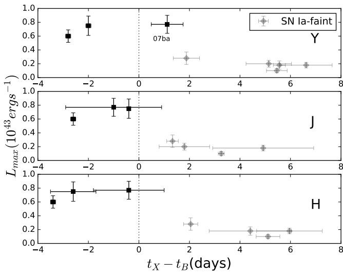
Fig. 2. Pseudo-bolometric peak luminosity versus the timing of the NIR ( YJH filters) maximum for SNe in our sample. SNe that peak earlier in the NIR (squares) than the optical also appear to be an extension to the normal SN Ia whereas all SNe with an NIR peak after the optical (diamonds) appear to be a distinct population in Fig. 1.
