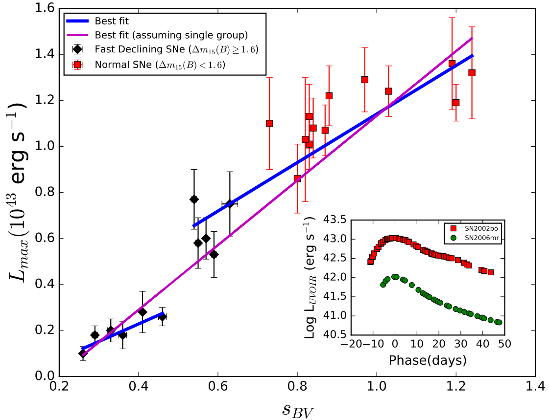
Fig. 1. L_{\max} versus s_{BV} for normal SNe Ia (red) and fast-declining SNe Ia (black). The best-fit linear relations for the faint sub-group of the fast-declining SNe Ia, the normal SNe, and the best-fit assuming that all SNe belong to the same group are plotted as solid lines. Inset: the u \rightarrow H pseudo-bolometric light curve for SN 2006mr (green), the faintest SN in the sample is plotted in comparison with the normal SN 2002bo (red, Benetti et al. 2004).
