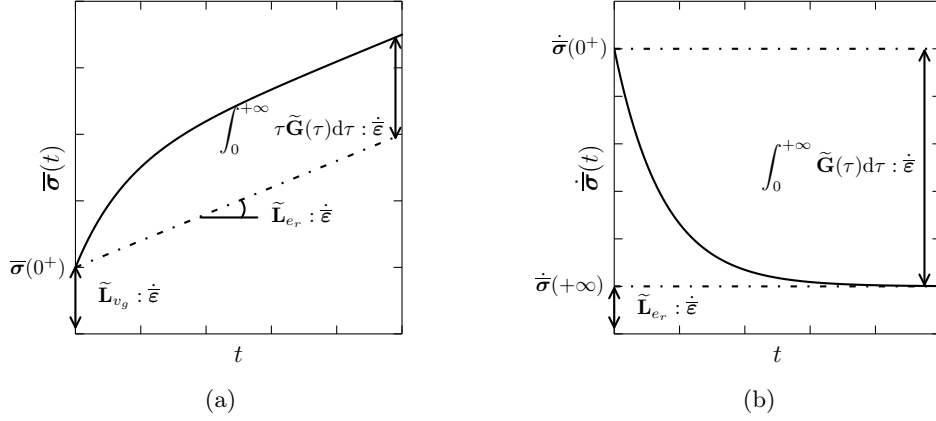
Figure 3: Physical interpretation on the overall relaxation spectrum \tilde{\mathbf{G}} for Type III viscoelastic behaviour. Stress and stress rate for a constant macroscopic strain rate \dot{\bar{\boldsymbol{\varepsilon}}} .
