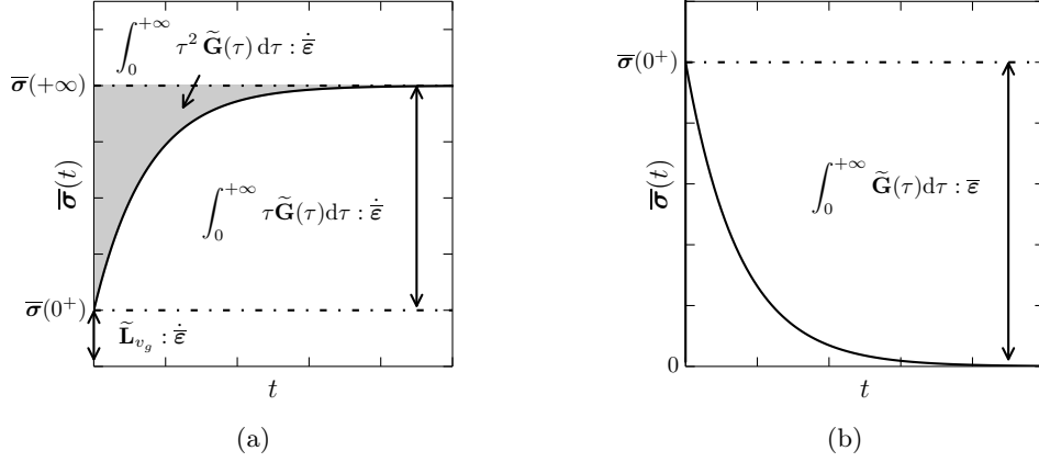
Figure 4: Physical interpretation on the overall relaxation spectrum \tilde{\mathbf{G}} for Type IV viscoelastic behaviour. (a): Stress response for a constant macroscopic strain rate \dot{\bar{\boldsymbol{\varepsilon}}} . (b): Relaxation stress for a constant macroscopic strain \bar{\boldsymbol{\varepsilon}} .
