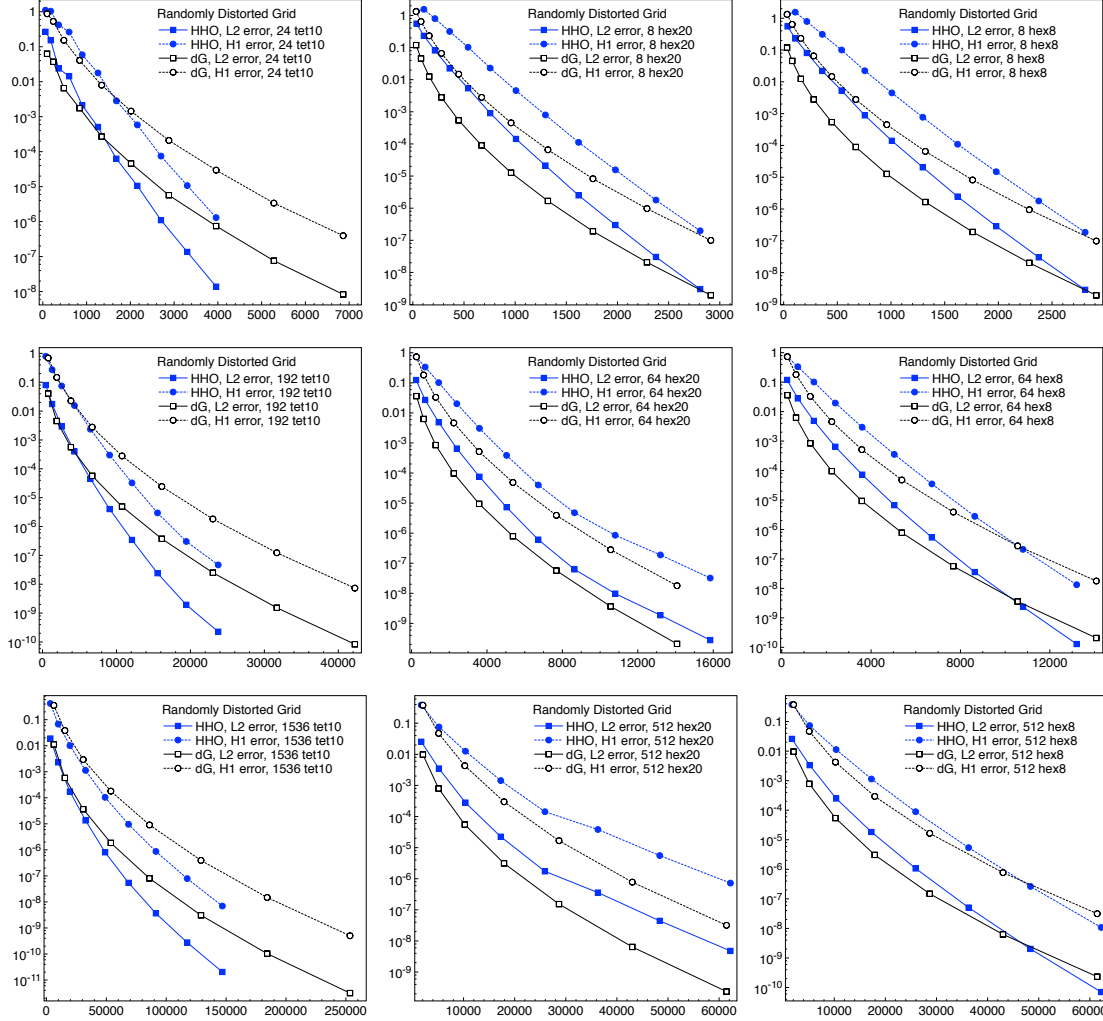
Figure 12: Error versus DOFs number. p -refined HHO and DG discretizations of the Poisson equation over the ten-nodes distorted tetrahedral meshes of Figure 2a (first column), the twenty-nodes distorted hexahedral meshes of Figure 2c (second column) and the eight-nodes distorted hexahedral meshes of Figure 2b (third column). HHO DOFs space is \underline{U}_h^{k,k} ( k = 0, 1, \dots ), DG DOFs space is \underline{U}_h^k ( k = 1, 2, \dots ).
