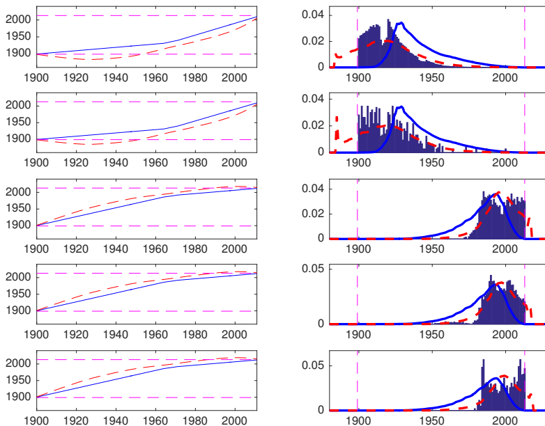
Figure 8: Children's first name at birth with support \Omega = [1900, 2013] . (Left) The dashed red curves represent the mapping \tilde{T}_i = \text{id} + \Pi_{\text{Sp}\{\tilde{u}_1\}}\omega_i where \omega_i = \log_{\bar{\nu}}(\nu_i) , and \tilde{u}_1 is the first principal direction in L^2_{\bar{\nu}}(\Omega) obtained via log-PCA. The blue curves are the mapping T_i = \text{id} + \Pi_{\text{Sp}\{u_1^*\}}\omega_i , where u_1^* is the first principal direction in L^2_{\bar{\nu}}(\Omega) obtained via the iterative algorithm. (Right) The histogram stands for the pdf of measures \nu_i that have a large Wasserstein distance with respect to the barycenter \bar{\nu} . The red curves are the pdf of the projection \exp_{\bar{\nu}}(\Pi_{\text{Sp}\{\tilde{u}_1\}}\omega_i) with log-PCA, while the blue curves are the pdf of the projection \exp_{\bar{\nu}}(\Pi_{\text{Sp}\{u_1^*\}}\omega_i) with GPCA.
