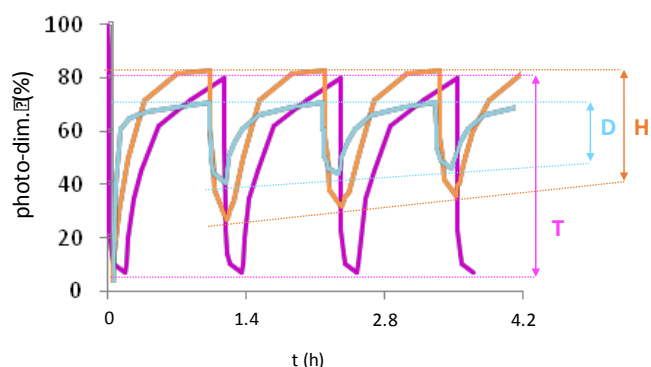
Figure 5: Photo-cycloaddition reversibility of NP_D , NP_H and NP_T after repetitive irradiation cycles at 350 nm (1 h) / 254 nm (10 min) (cycloaddition/cleavage) for the two first and 254 (10 min) / 350 nm (1 h) (cleavage/cycloaddition) for the last.
