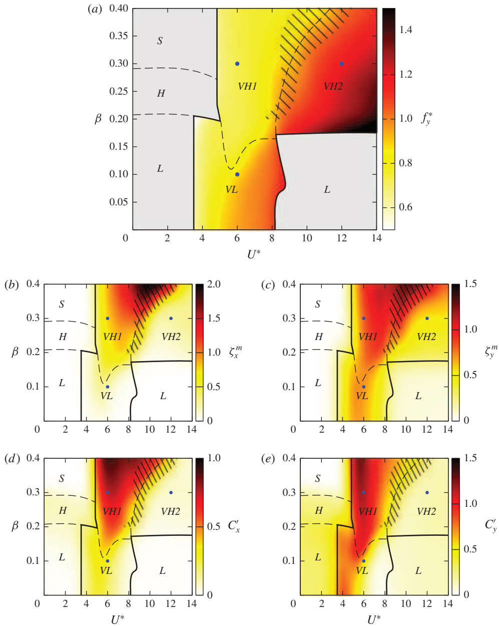
FIGURE 10. (Colour online) Flow–structure interaction regimes: iso-contours of (a) f_y^* , (b) \zeta_x^m , (c) \zeta_y^m , (d) C'_x and (e) C'_y , in the (\beta, U^*) parameter space. In each plot, the map of the flow–structure interaction regimes is overlaid on the iso-contours. A plain black line delimitates the large-amplitude vibration region. A striped area indicates the region of irregular responses studied in §4.2.3. Blue symbols denote the points examined in figures 12, 14 and 15.
